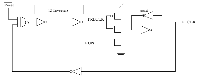
Fig. 4. Our basic stoppable ring oscillator clock.
