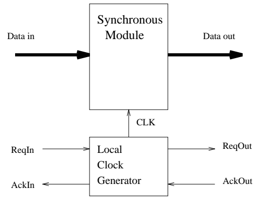
Fig. 2. Basic module of a GALS architecture.
