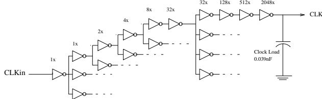
Fig. 11. Clock buffer tree model simulated in HSPICE.
