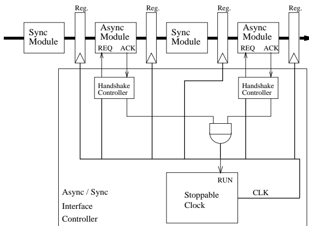
Fig. 3. Proposed interface methodology.
