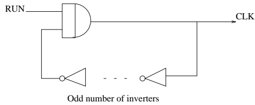
Fig. 1. A stoppable ring oscillator clock.
