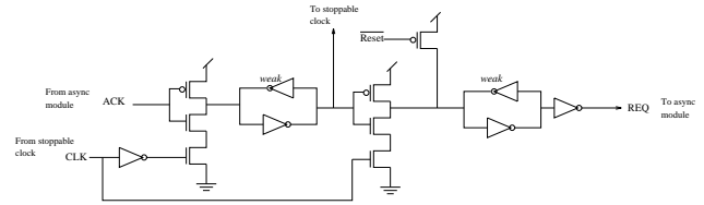
Fig. 6. Handshake control circuit with conditioned acknowledgment.
