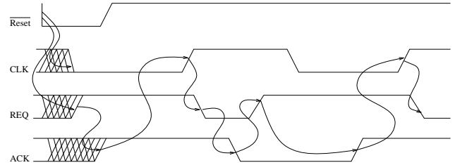
Fig. 7. Idealized waveform for the basic interface controller.
