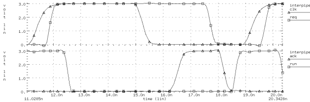
Fig. 17. HSPICE results for the pipelined interface controller design.
