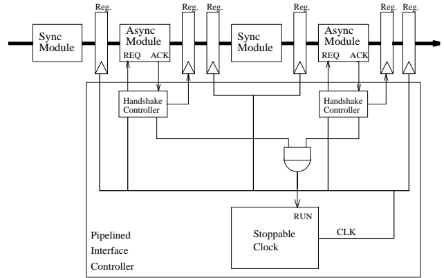
Fig. 15. Interface controller with pipeline latch.
