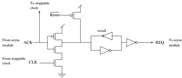
Fig. 5. Handshake control circuit.
