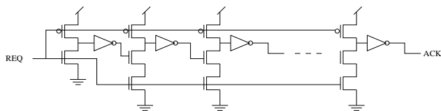
Fig. 8. Domino buffer chain used to model the datapath.
