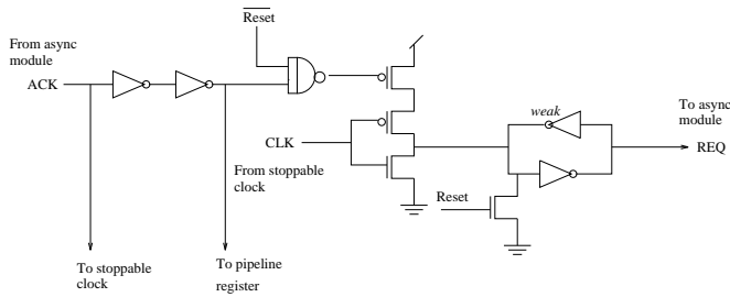
Fig. 16. New handshake control circuit.
