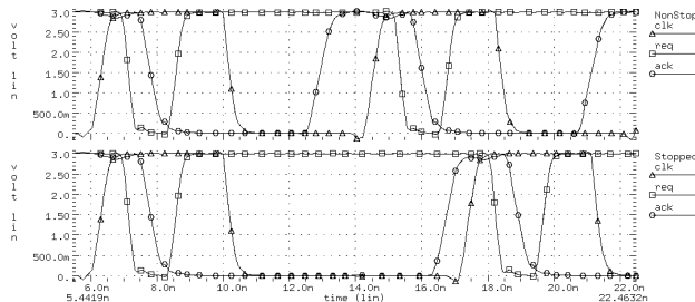
Fig. 9. HSPICE results for the basic interface controller.
