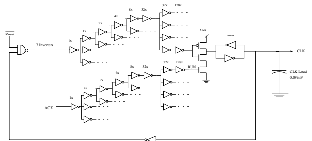
Fig. 13. Stoppable ring oscillator clock with buffering.
